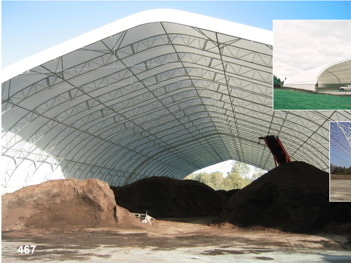
DAVISON FARMS, Maple Ridge – Dairy Manure Composting LP 80 X 200
